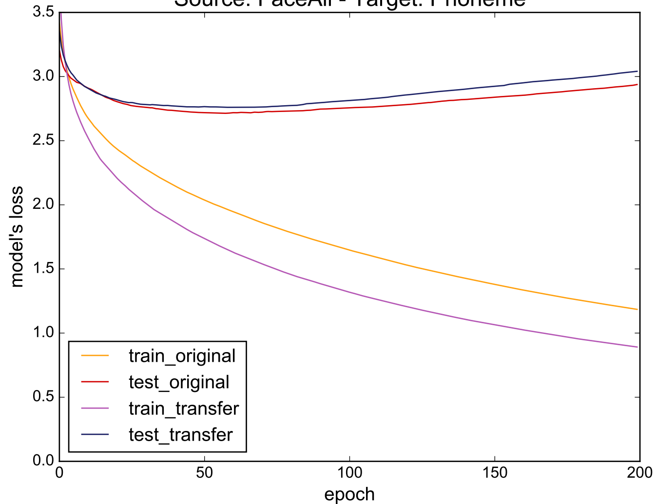
Source: FaceAll - Target: Phoneme
