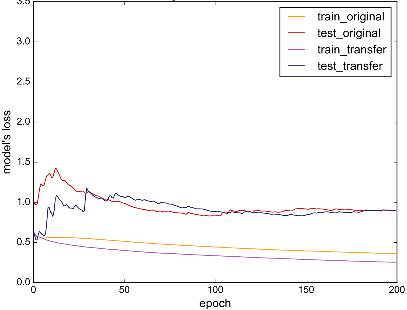
Source: FaceAll - Target: ProximalPhalanxOutlineCorrect
