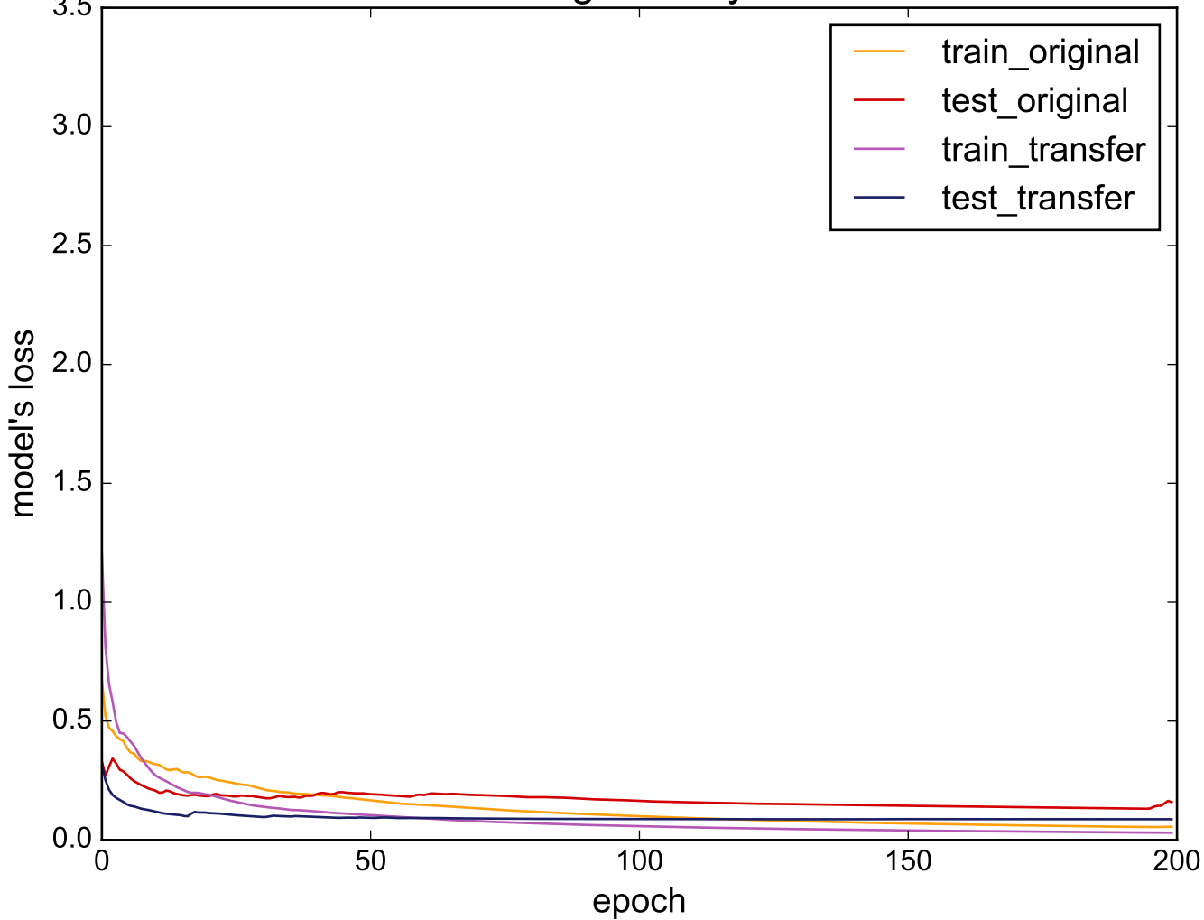
Source: FaceAll - Target: SonyAIBORobotSurface
