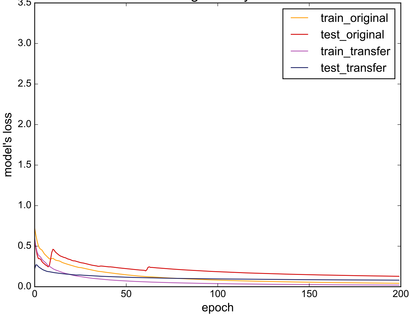
Source: FaceAll - Target: SonyAIBORobotSurfacell
