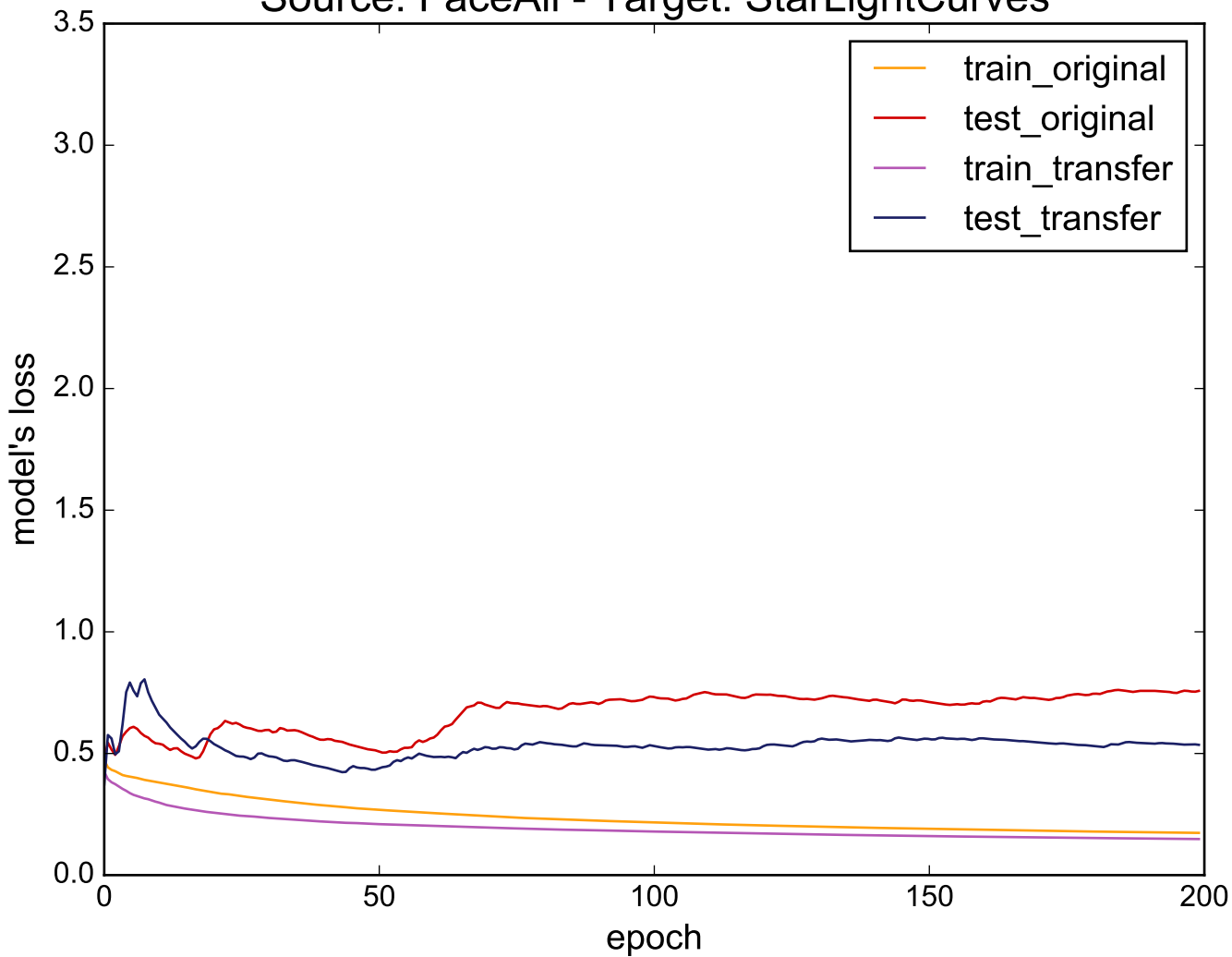
Source: FaceAll - Target: StarLightCurves
