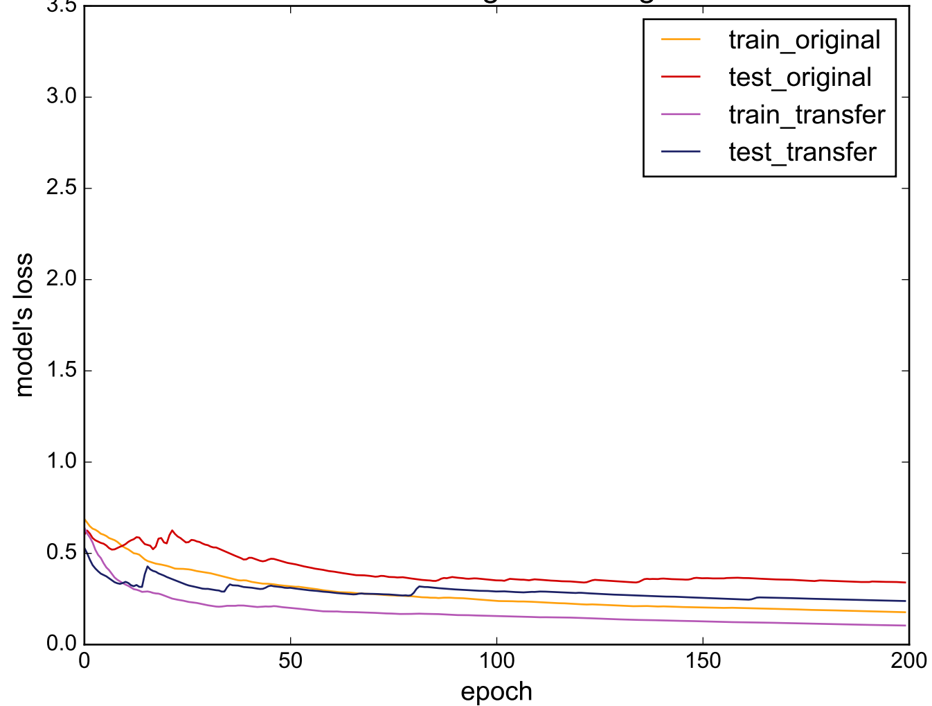
Source: FaceAll - Target: ToeSegmentation1
