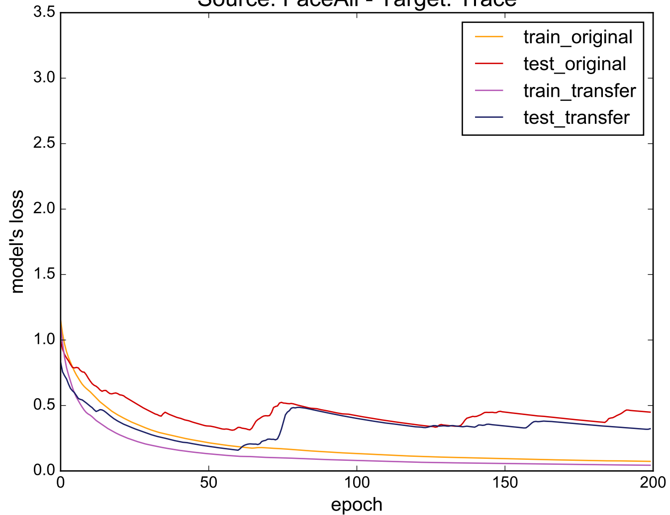
Source: FaceAll - Target: Trace
