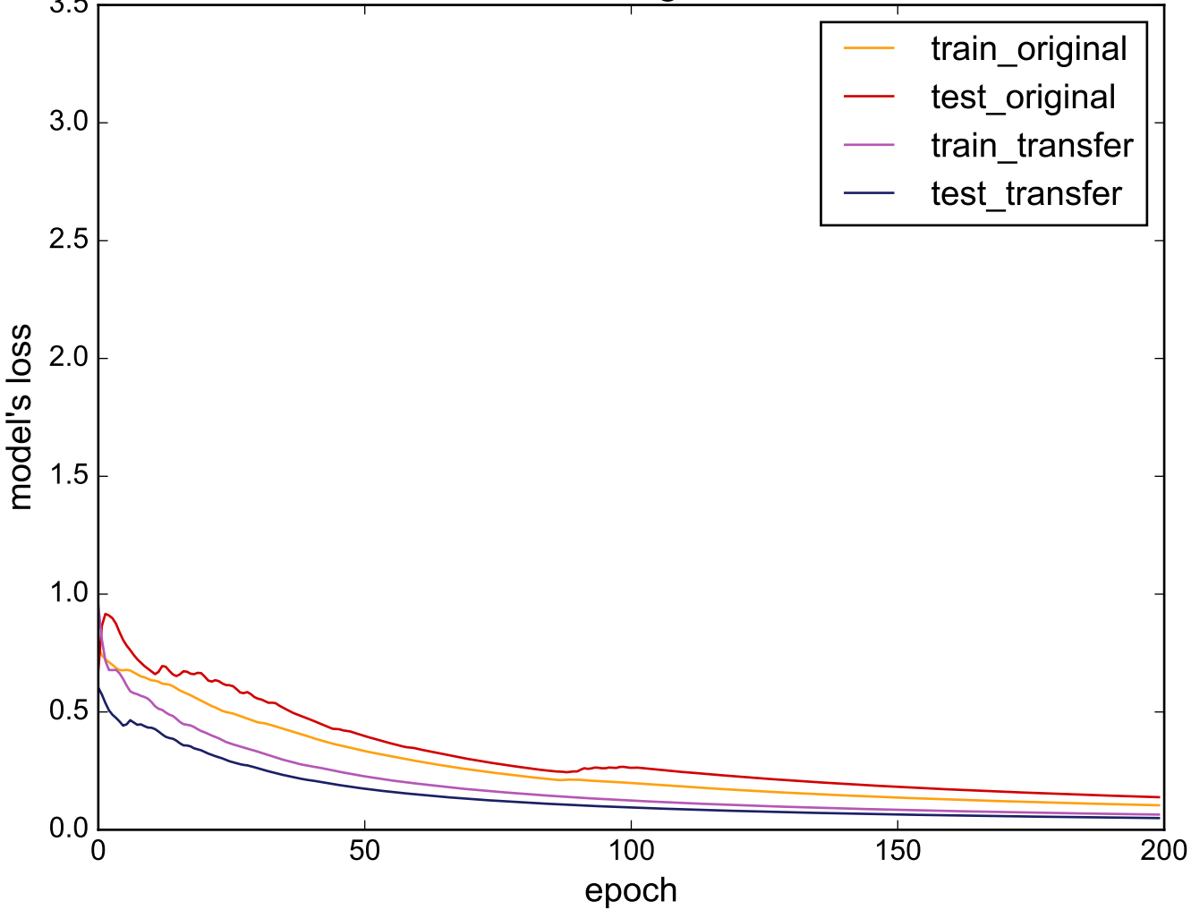
Source: FaceAll - Target: TwoLeadECG
