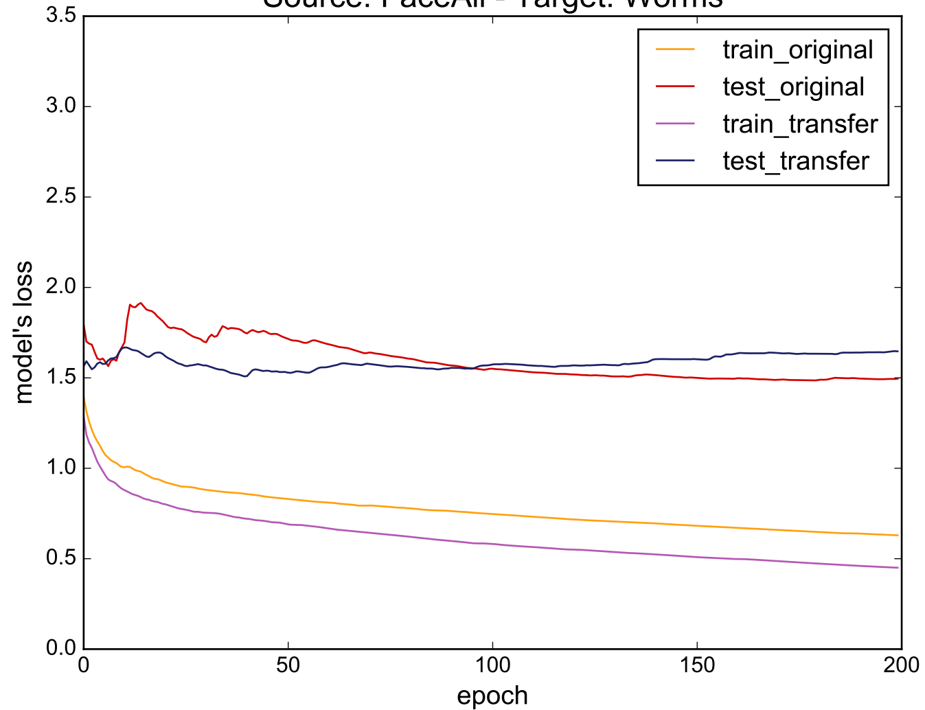
Source: FaceAll - Target: Worms
