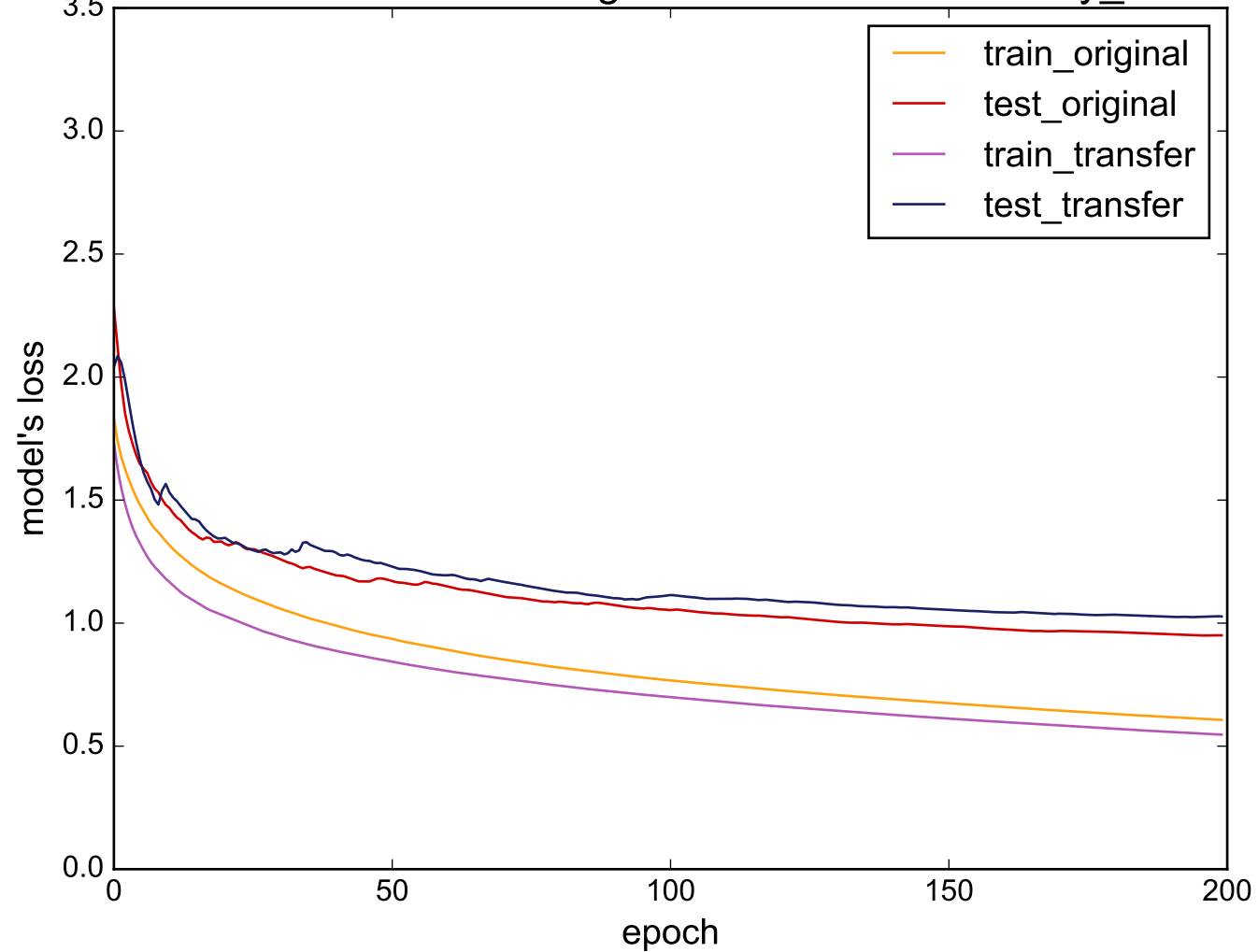
Source: FaceAll - Target: uWaveGestureLibrary_X
