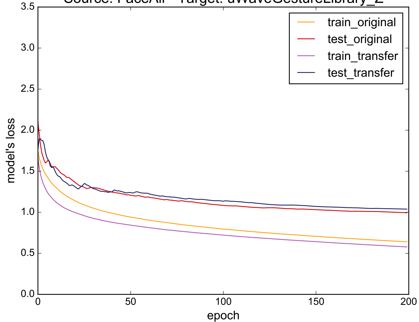
Source: FaceAll - Target: uWaveGestureLibrary_Z
