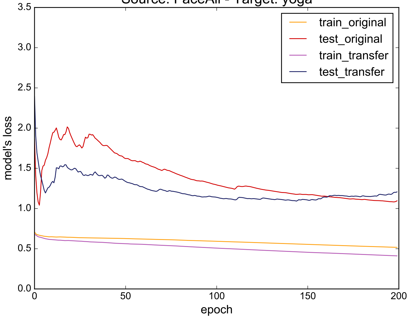
Source: FaceAll - Target: yoga
