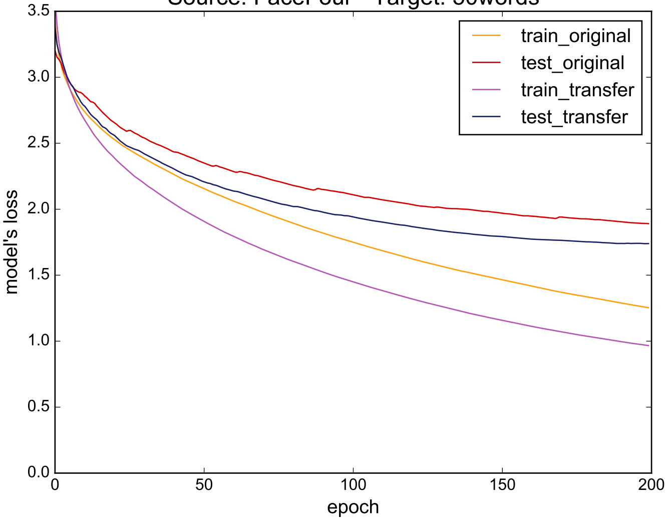
Source: FaceFour - Target: 50words
