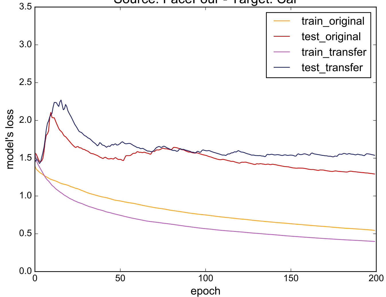
Source: FaceFour - Target: Car
