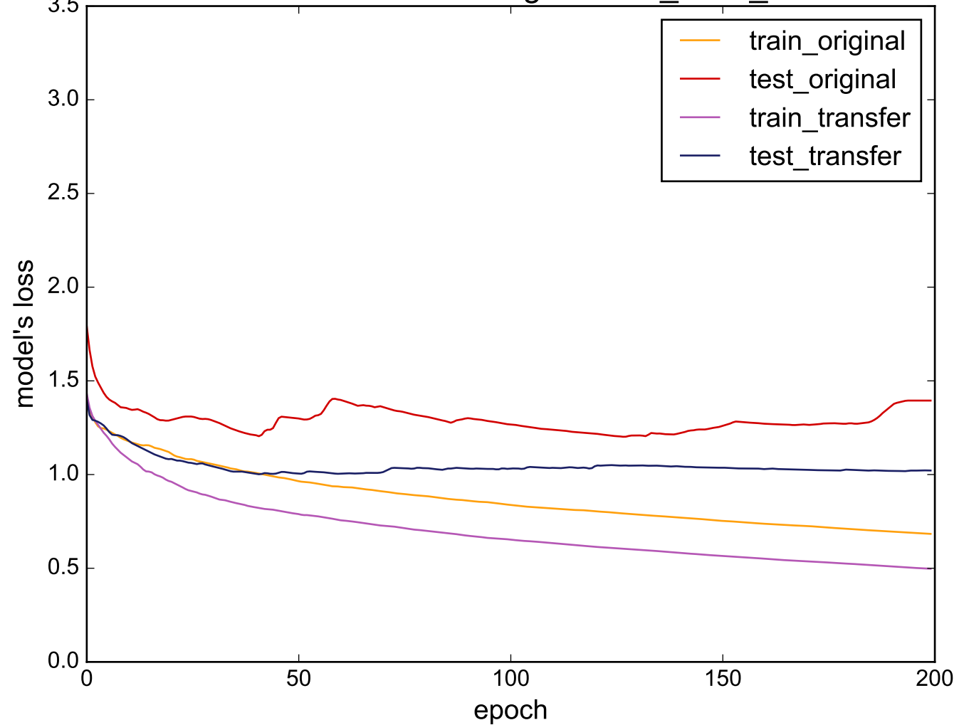
Source: FaceFour - Target: CinC_ECG_torso
