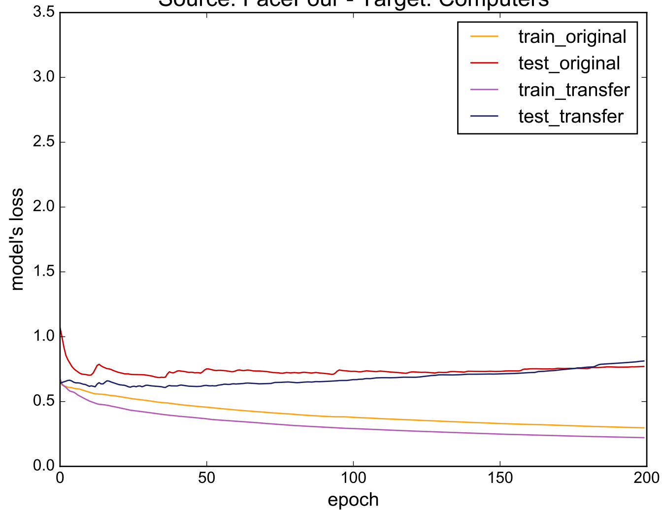
Source: FaceFour - Target: Computers
