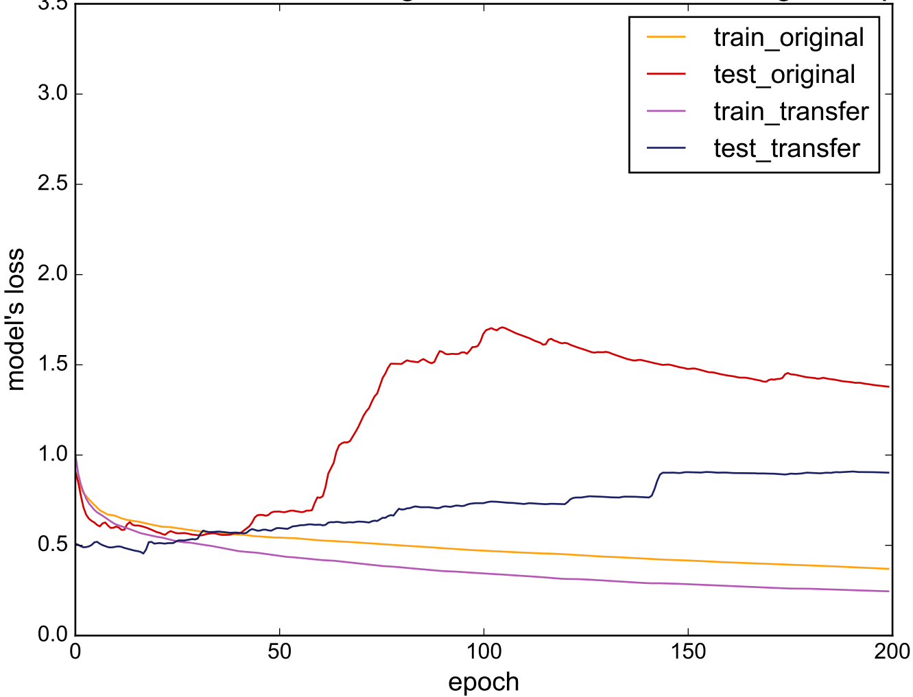
Source: FaceFour - Target: DistalPhalanxOutlineAgeGroup
