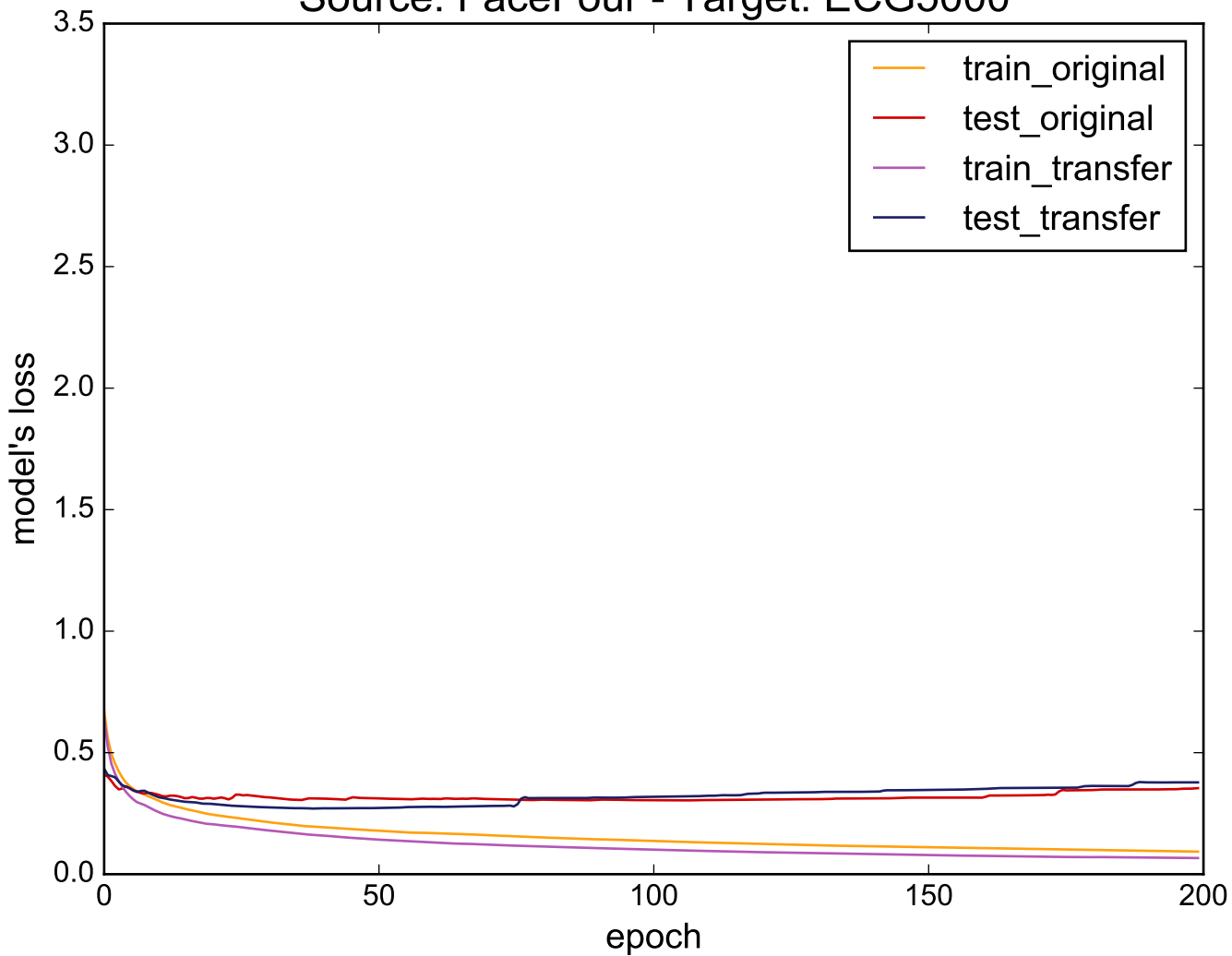
Source: FaceFour - Target: ECG5000
