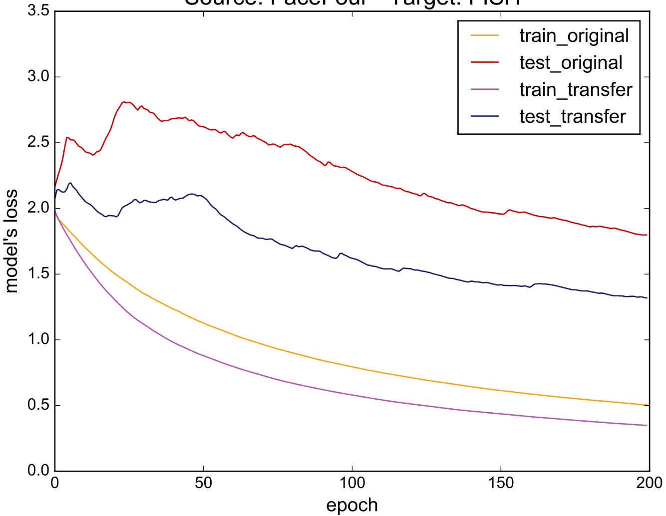
Source: FaceFour - Target: FISH
