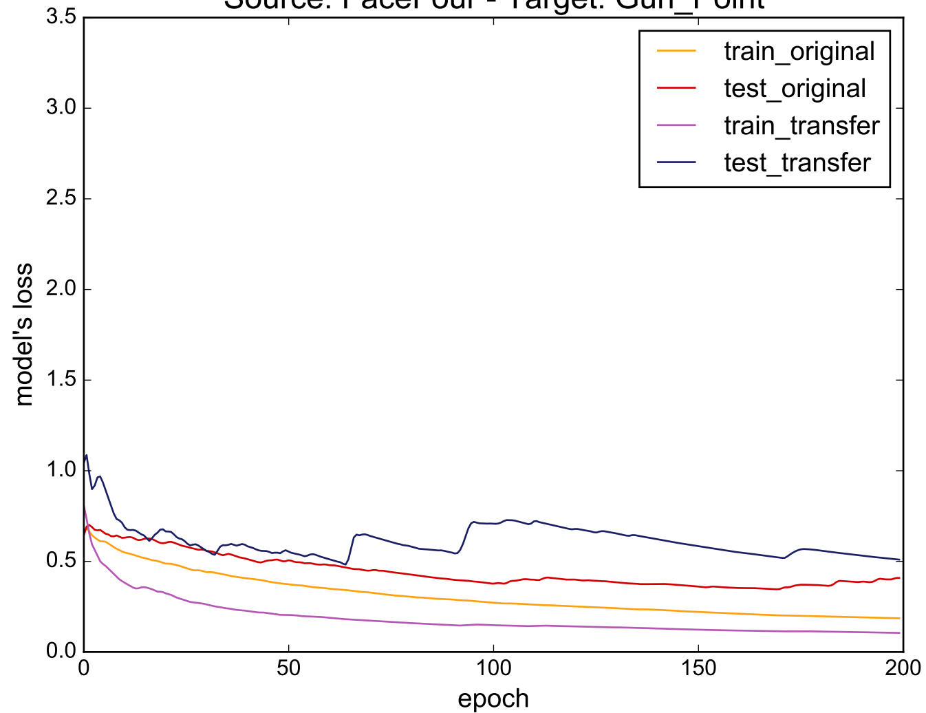
Source: FaceFour - Target: Gun_Point
