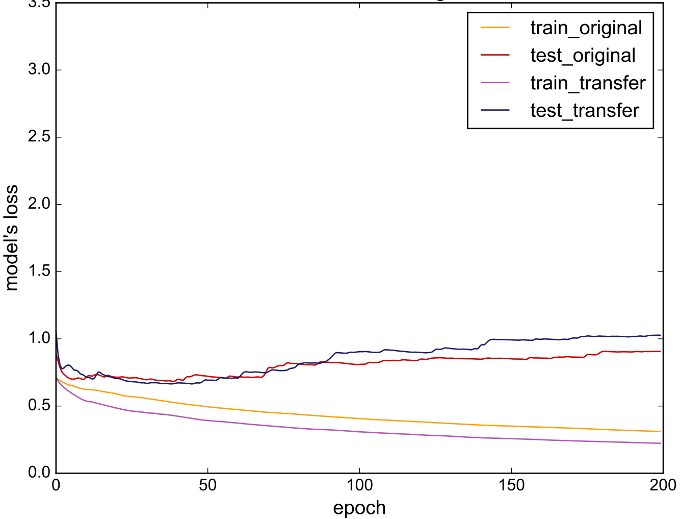
Source: FaceFour - Target: Ham
