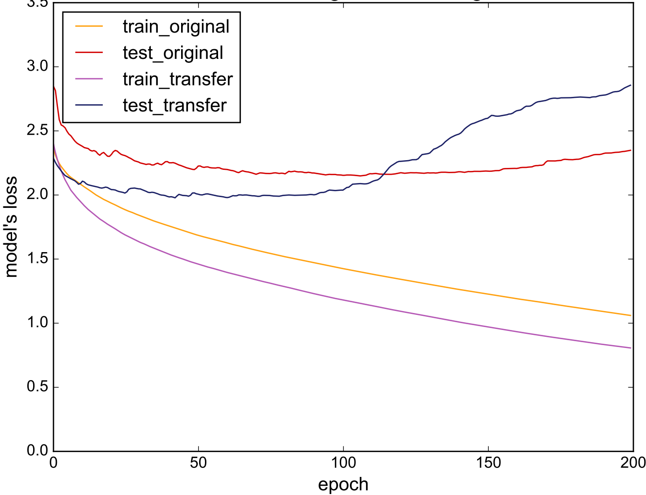
Source: FaceFour - Target: InsectWingbeatSound
