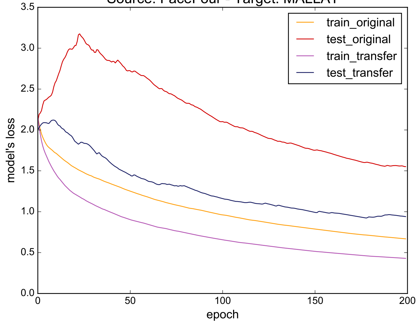
Source: FaceFour - Target: MALLAT
