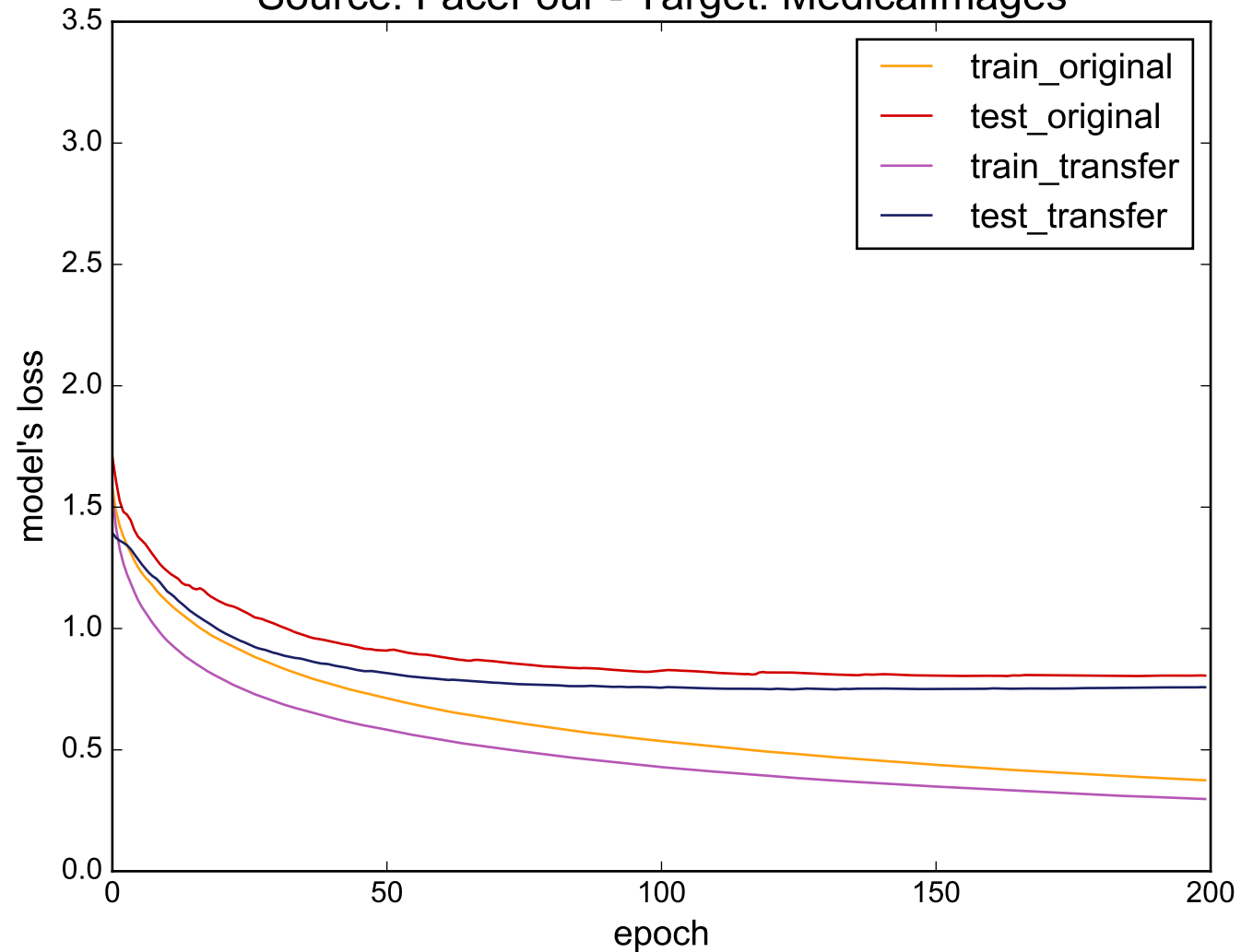
Source: FaceFour - Target: MedicalImages
