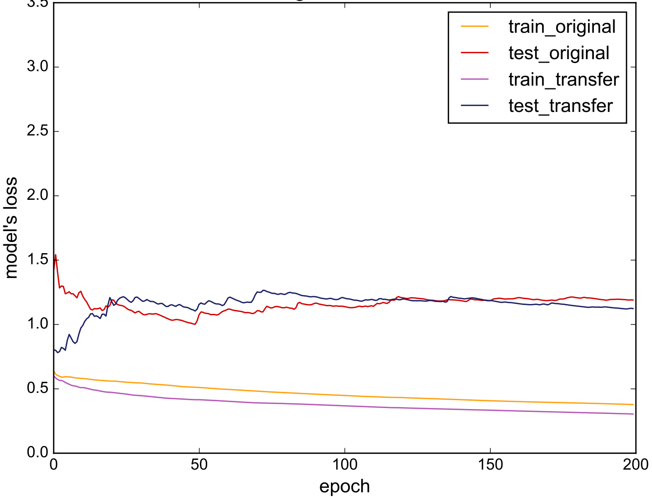
Source: FaceFour - Target: MiddlePhalanxOutlineCorrect
