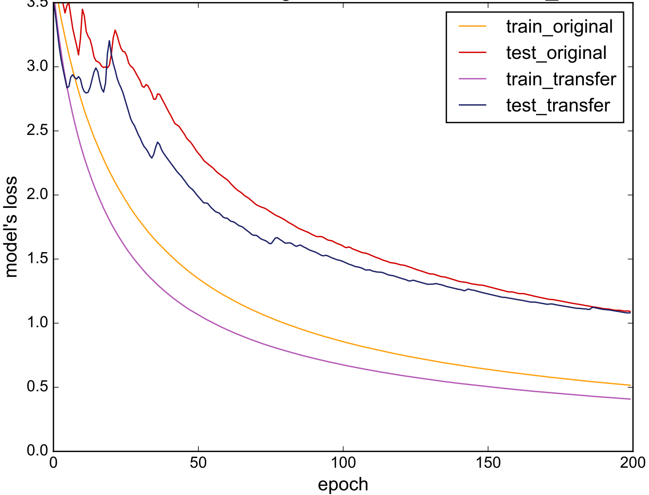
Source: FaceFour - Target: NonInvasiveFataLECG_Thorax1
