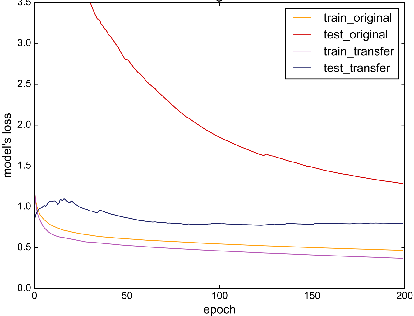
Source: FaceFour - Target: ProximalPhalanxTW
