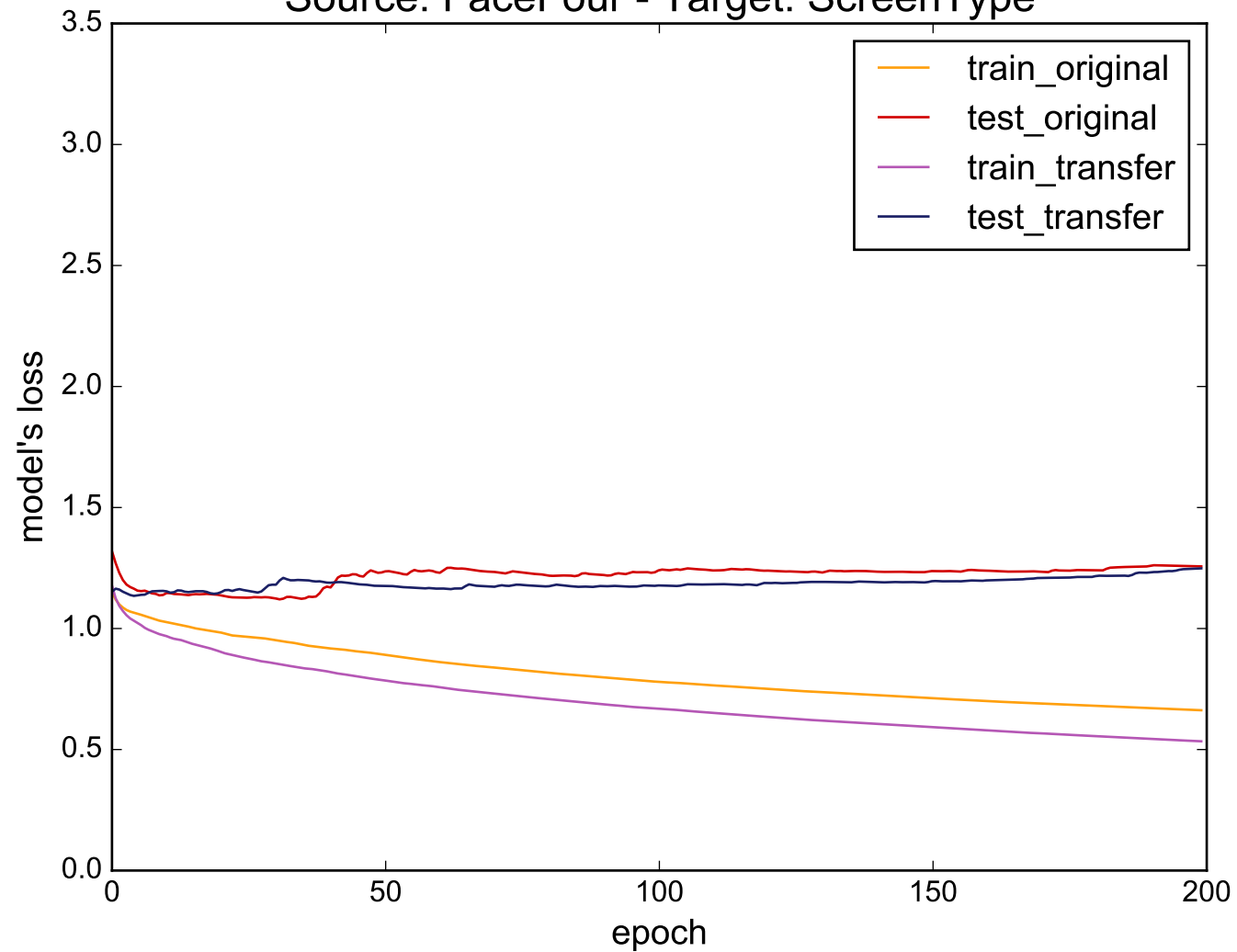
Source: FaceFour - Target: ScreenType
