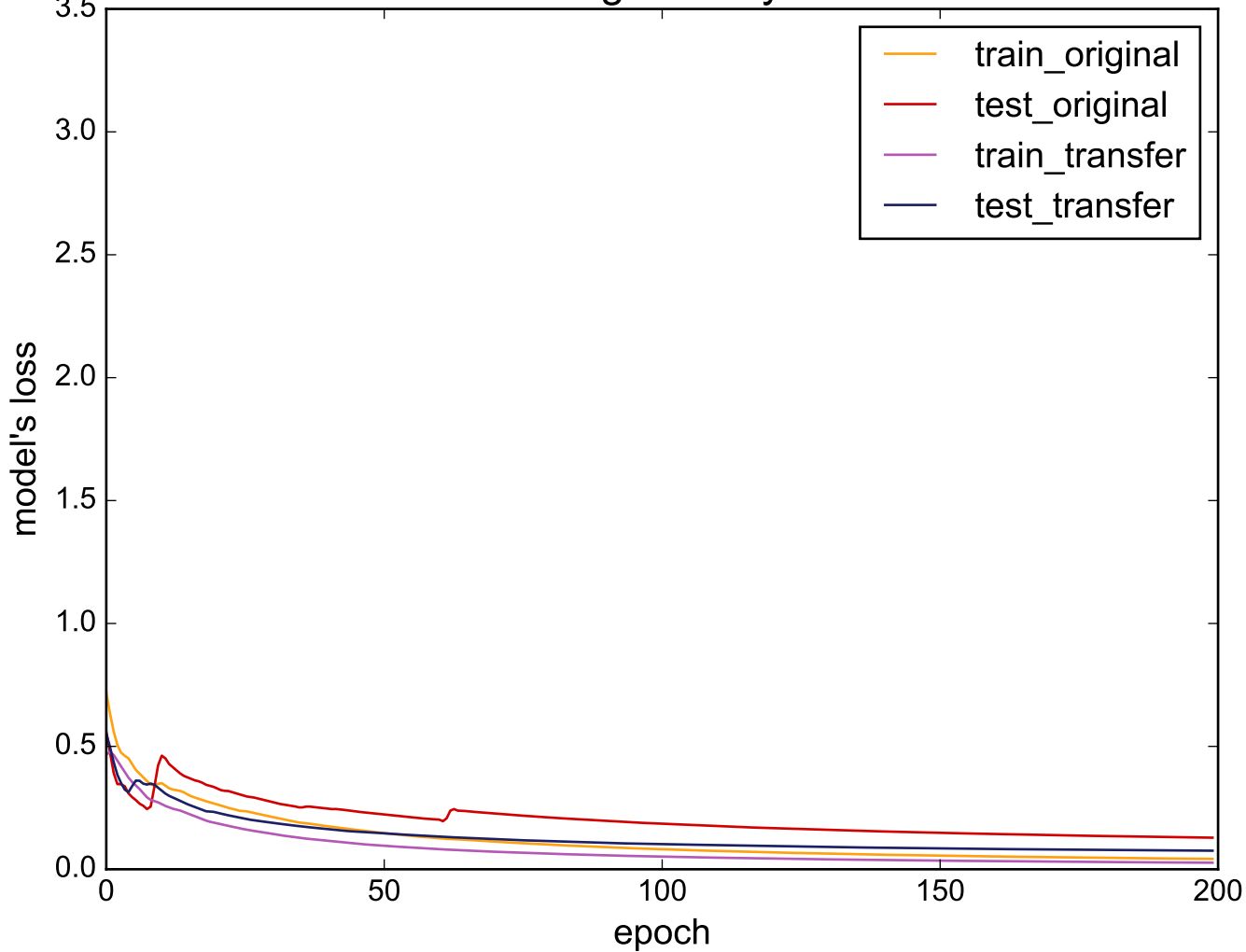
Source: FaceFour - Target: SonyAIBORobotSurfacell
