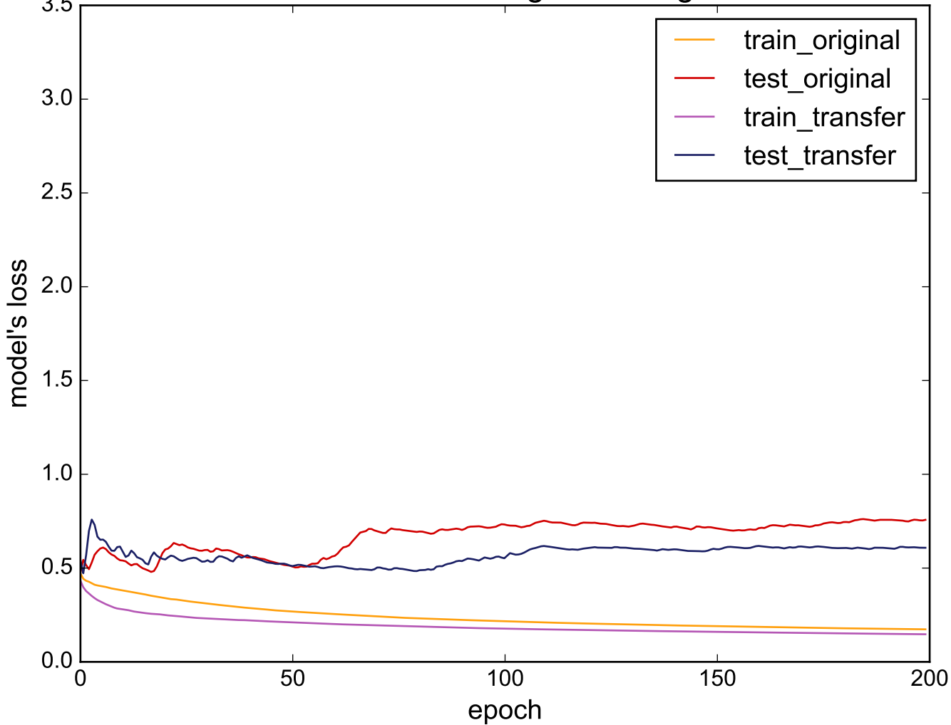
Source: FaceFour - Target: StarLightCurves
