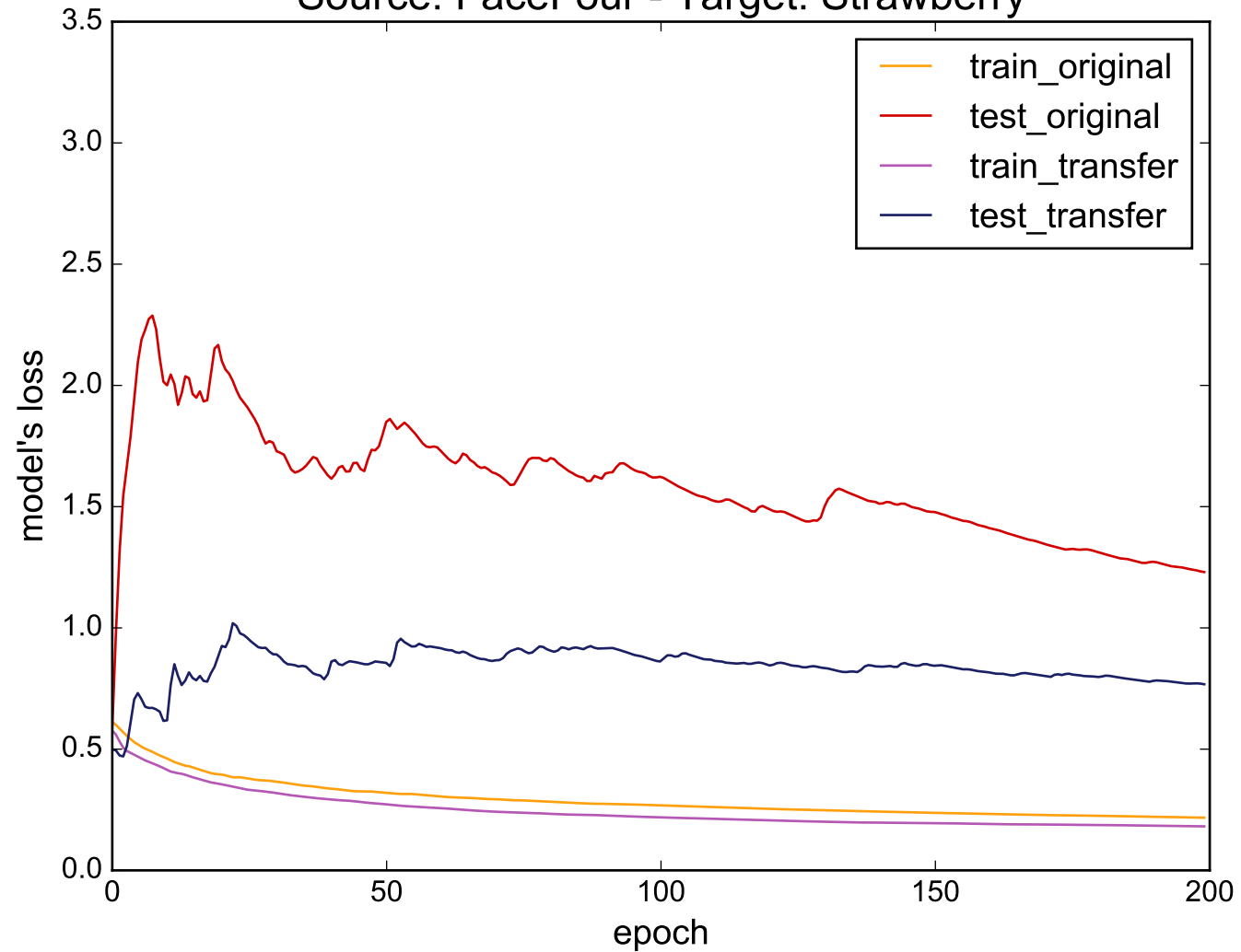
Source: FaceFour - Target: Strawberry
