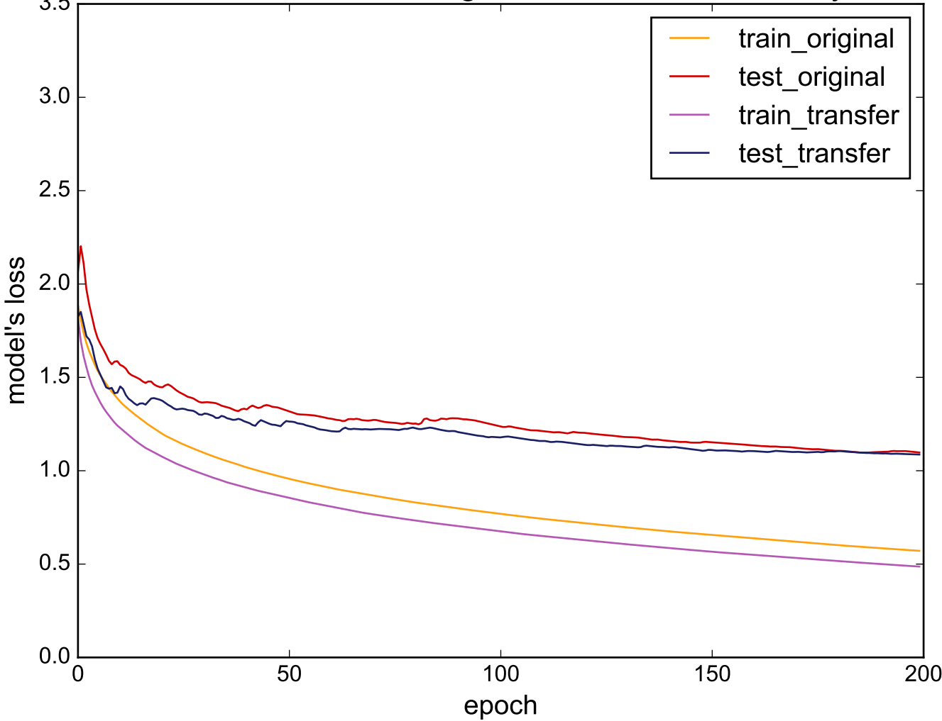
Source: FaceFour - Target: UWaveGestureLibraryAll
