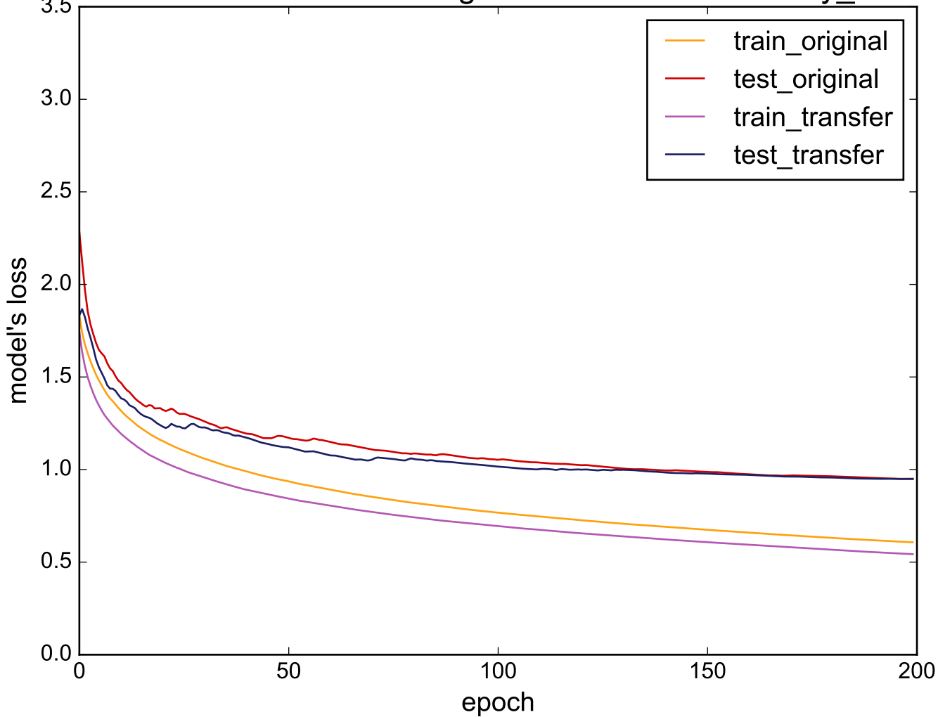
Source: FaceFour - Target: uWaveGestureLibrary_X
