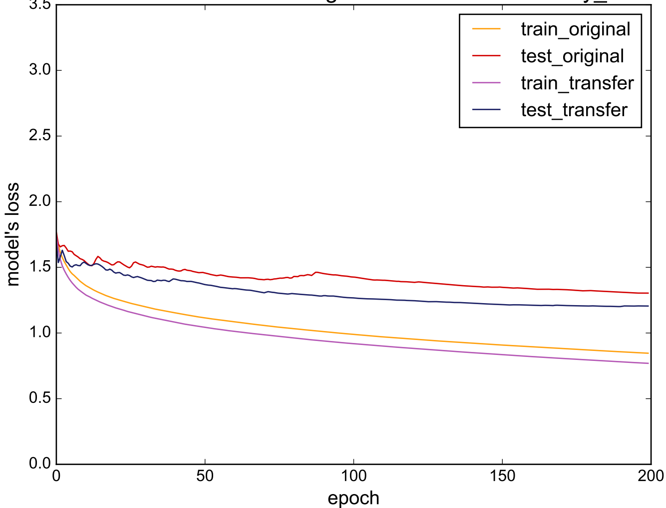
Source: FaceFour - Target: uWaveGestureLibrary_Y
