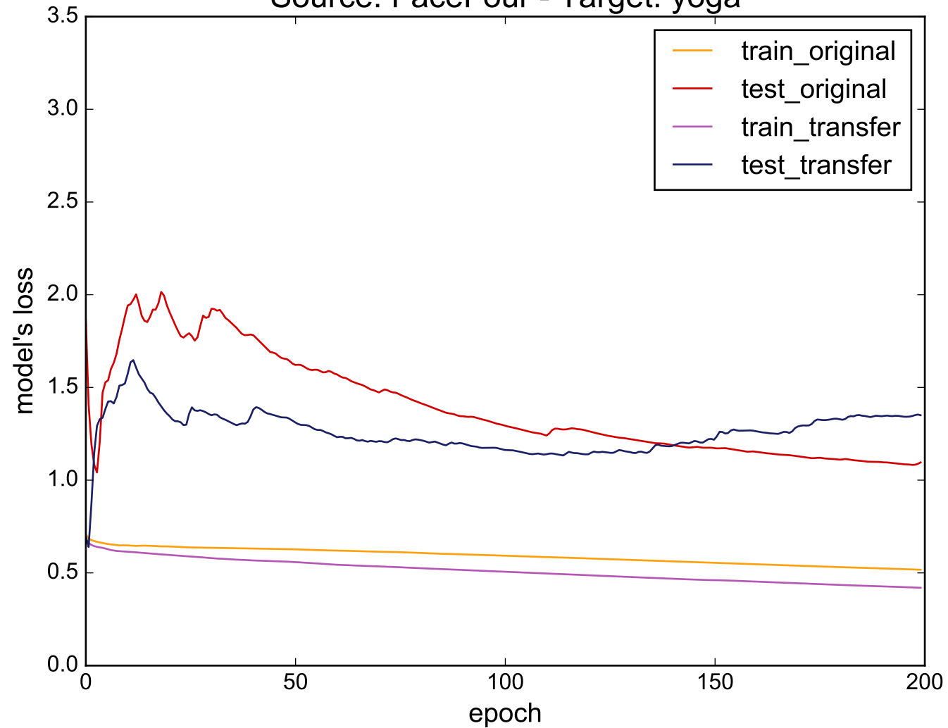
Source: FaceFour - Target: yoga
