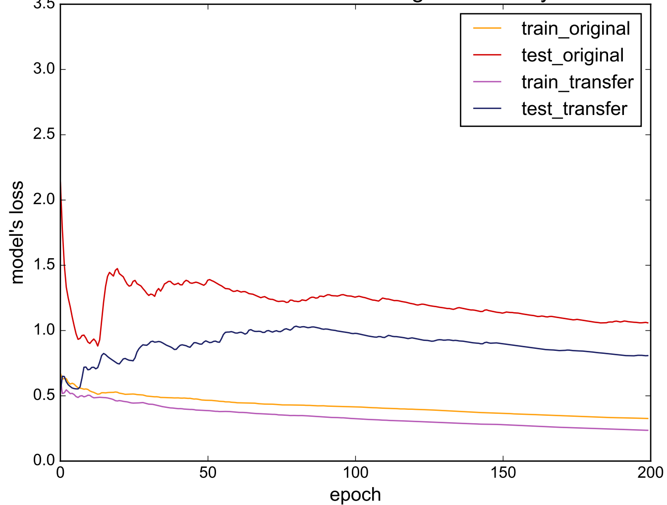
Source: FacesUCR - Target: BeetleFly
