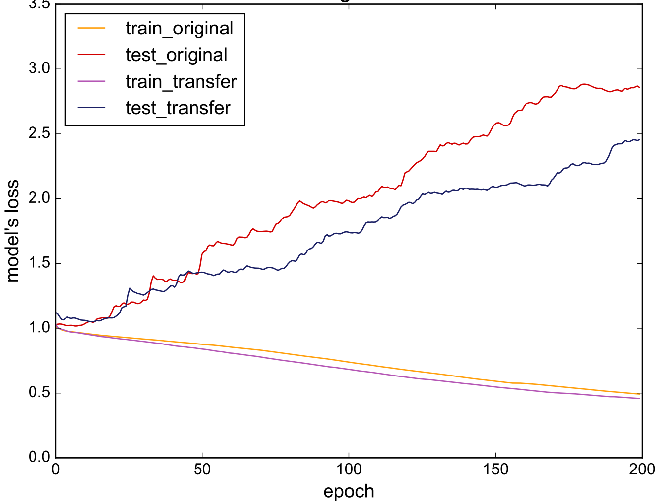
Source: FacesUCR - Target: ChlorineConcentration
