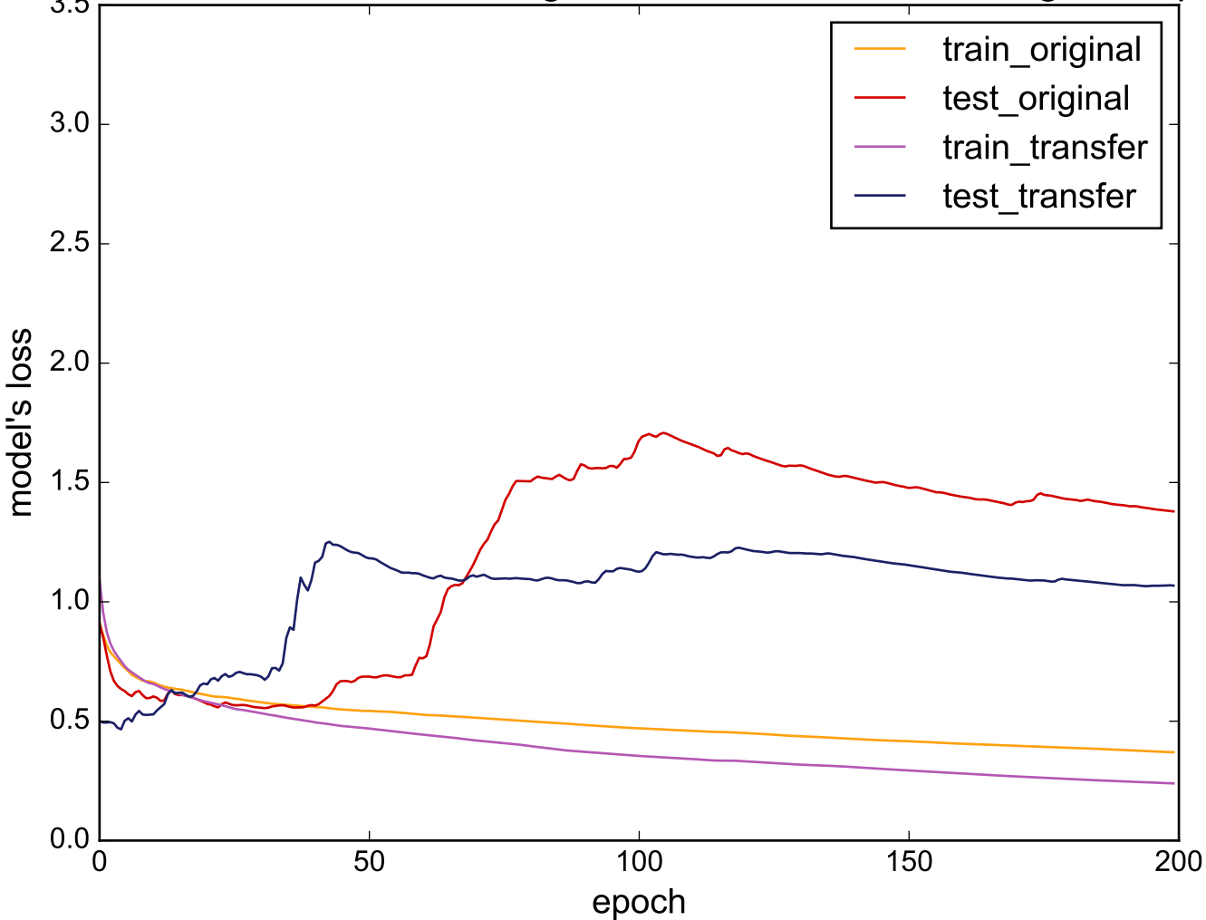
Source: FacesUCR - Target: DistalPhalanxOutlineAgeGroup
