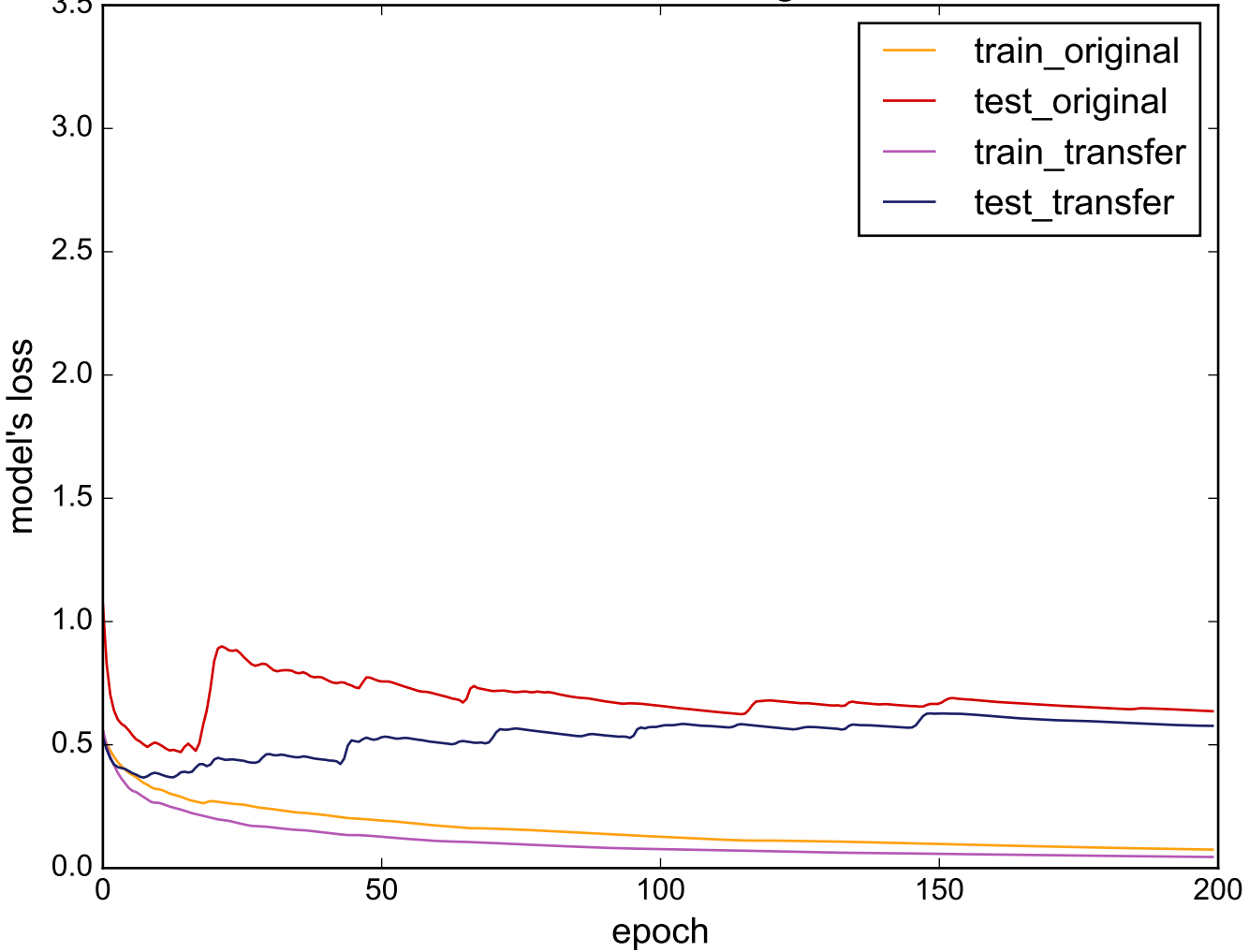
Source: FacesUCR - Target: ECG200
