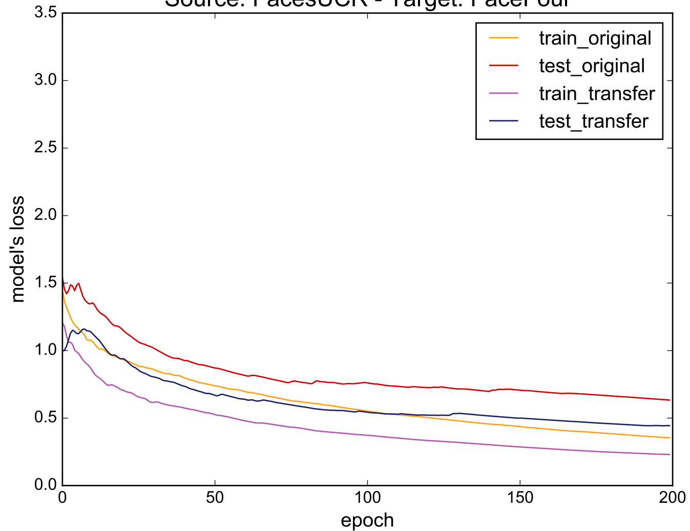
Source: FacesUCR - Target: FaceFour
