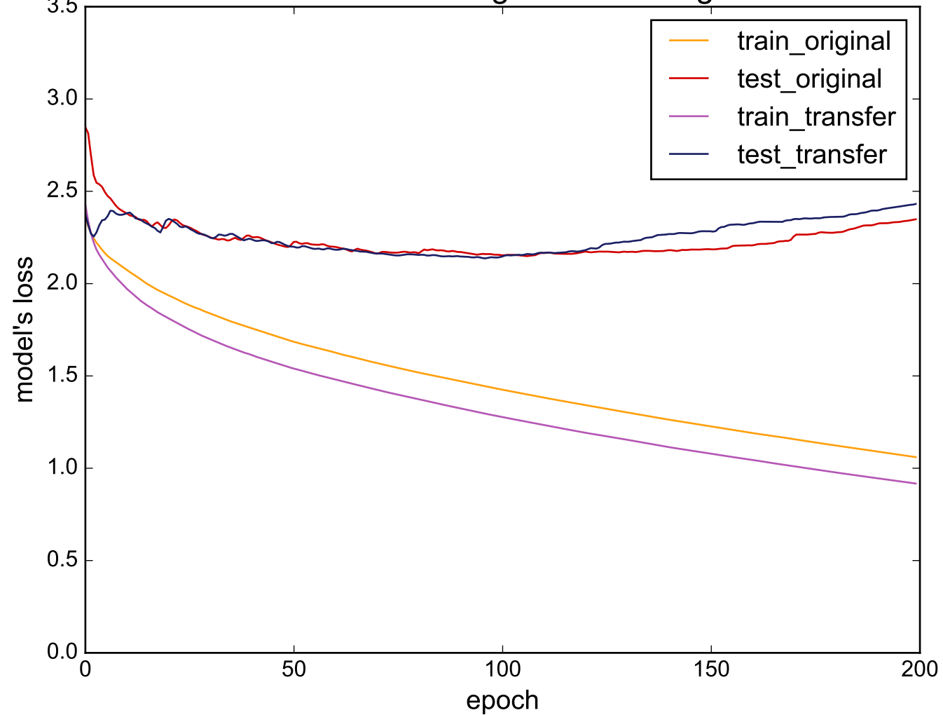
Source: FacesUCR - Target: InsectWingbeatSound
