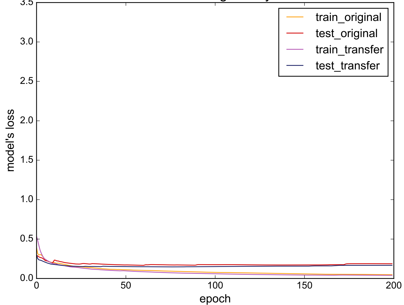
Source: FacesUCR - Target: ItalyPowerDemand
