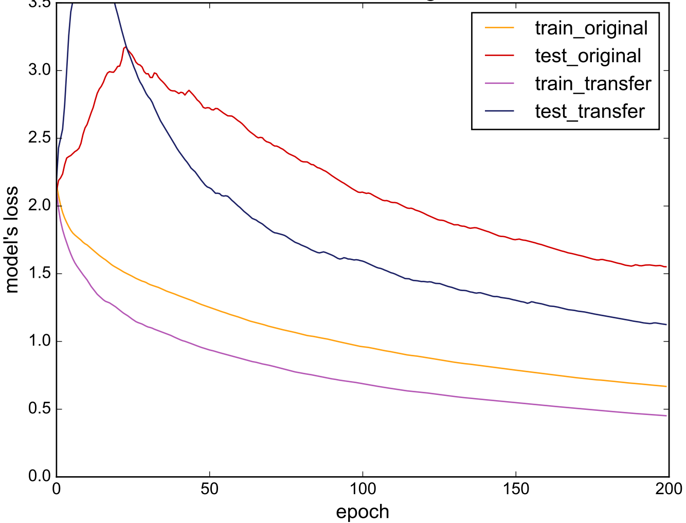
Source: FacesUCR - Target: MALLAT
