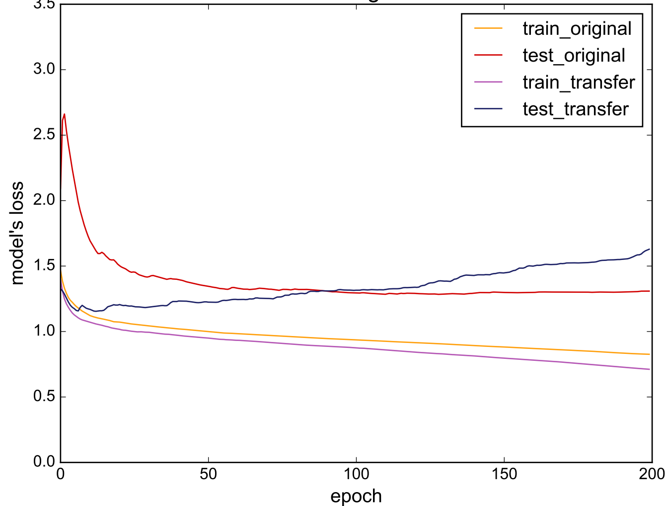
Source: FacesUCR - Target: MiddlePhalanxTW
