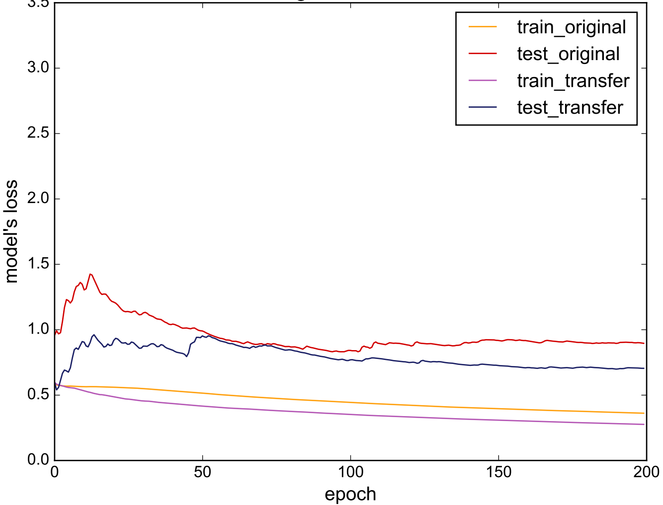
Source: FacesUCR - Target: ProximalPhalanxOutlineCorrect
