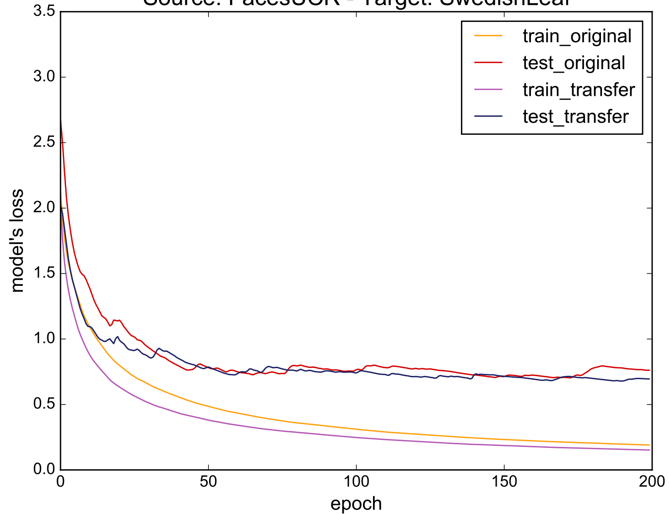
Source: FacesUCR - Target: SwedishLeaf
