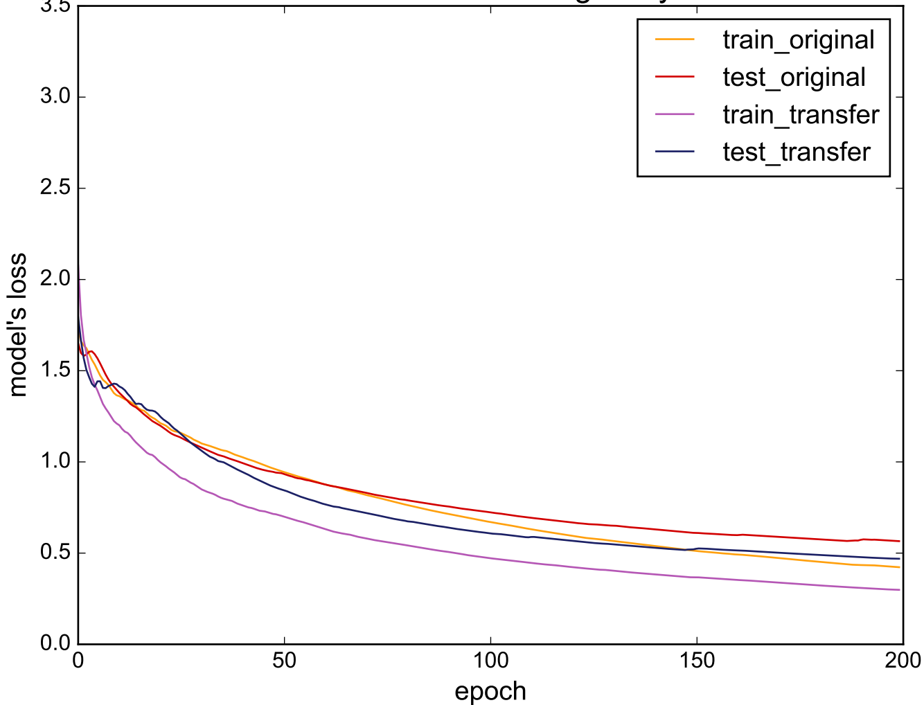
Source: FacesUCR - Target: Symbols
