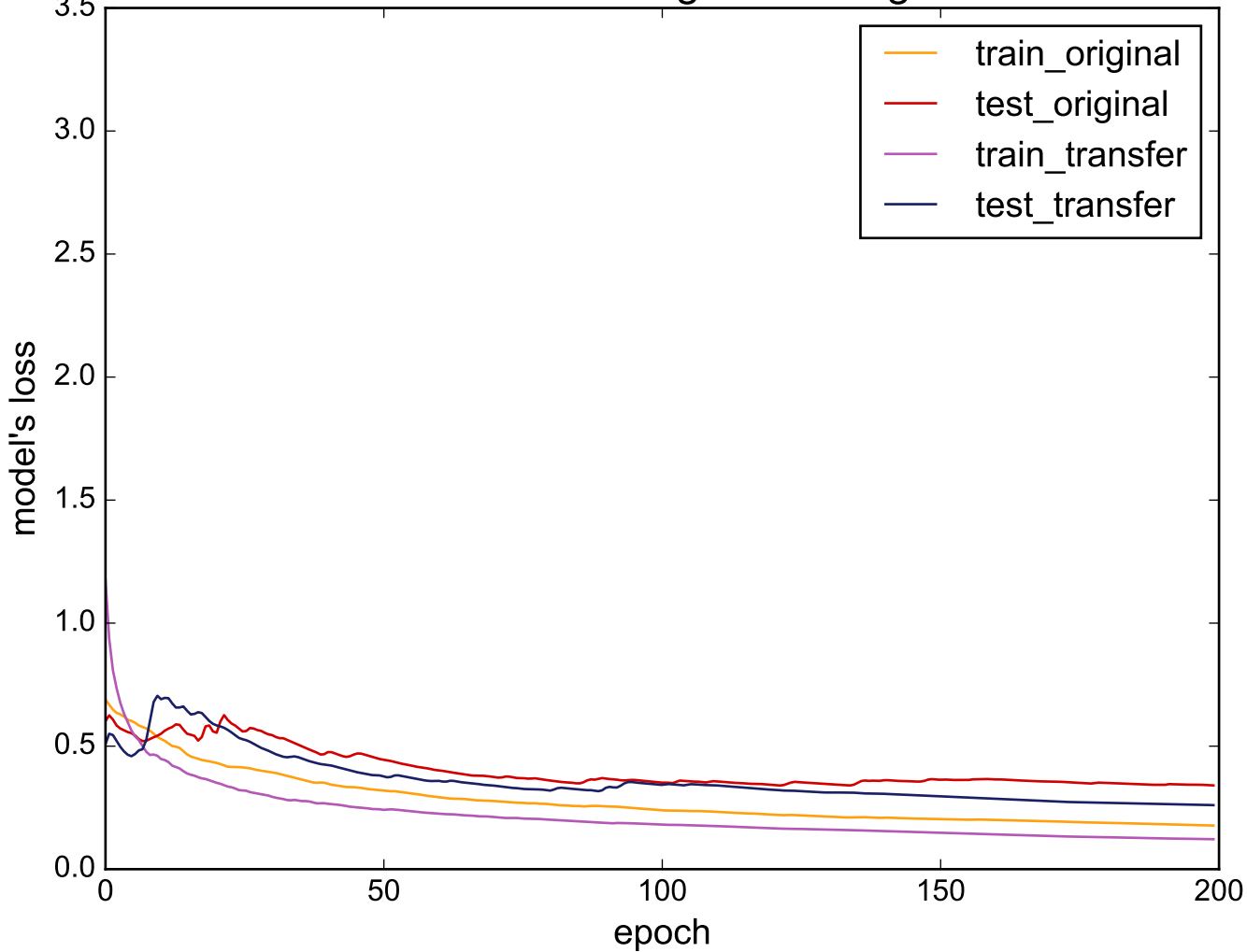
Source: FacesUCR - Target: ToeSegmentation1
