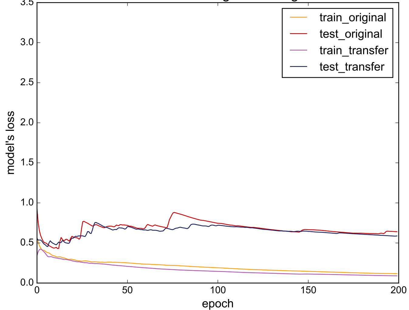
Source: FacesUCR - Target: ToeSegmentation2
