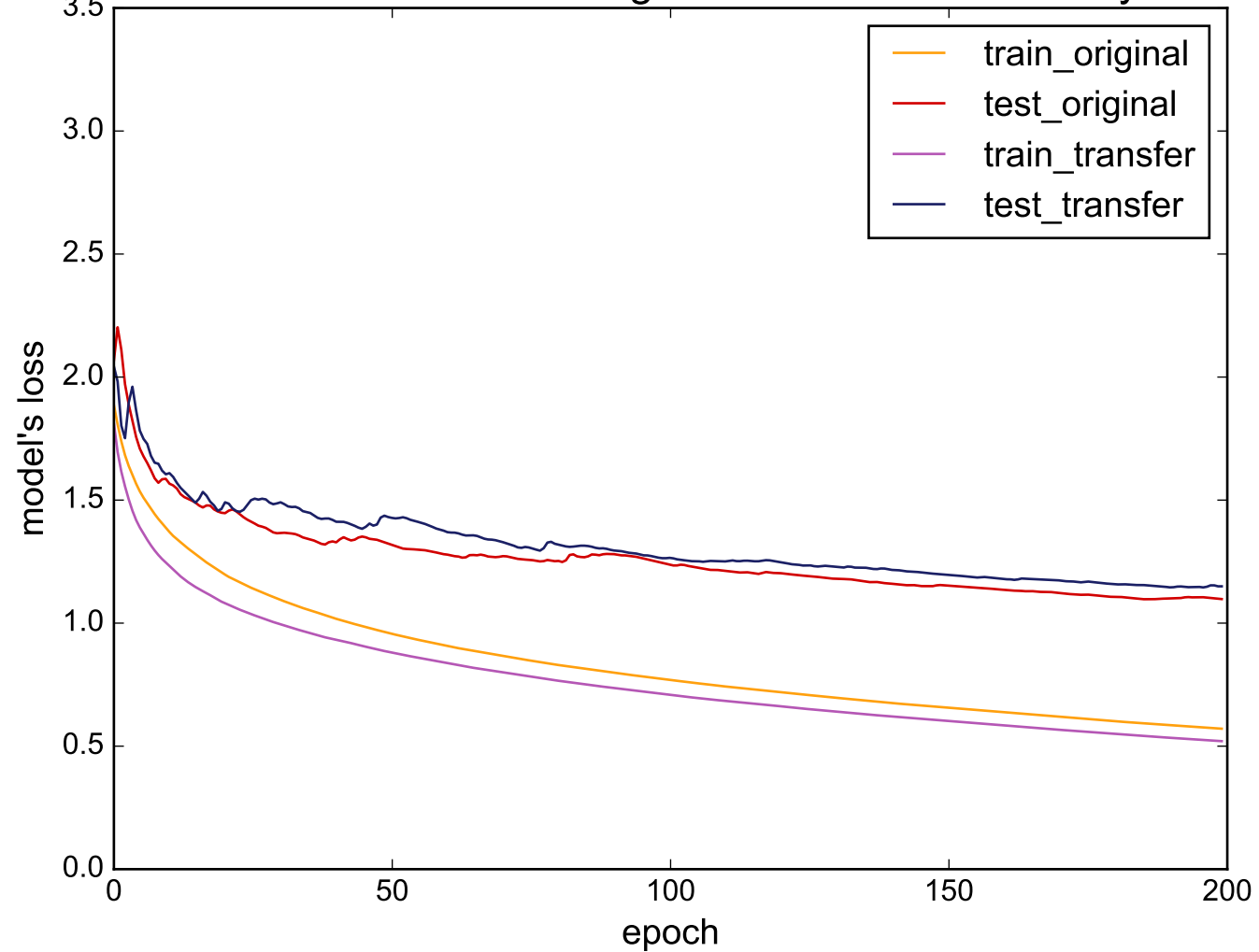
Source: FacesUCR - Target: UWaveGestureLibraryAll
